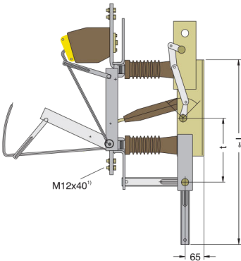
Type H 22 EA with earthing switch mounted below
